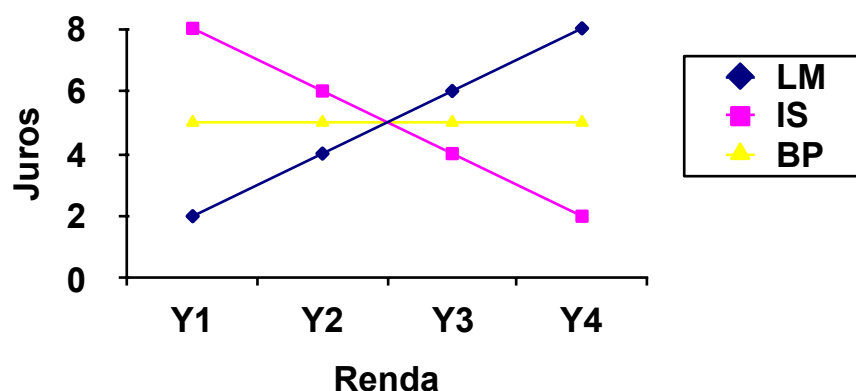
Figura 9.1: Curvas IS-LM-BP
